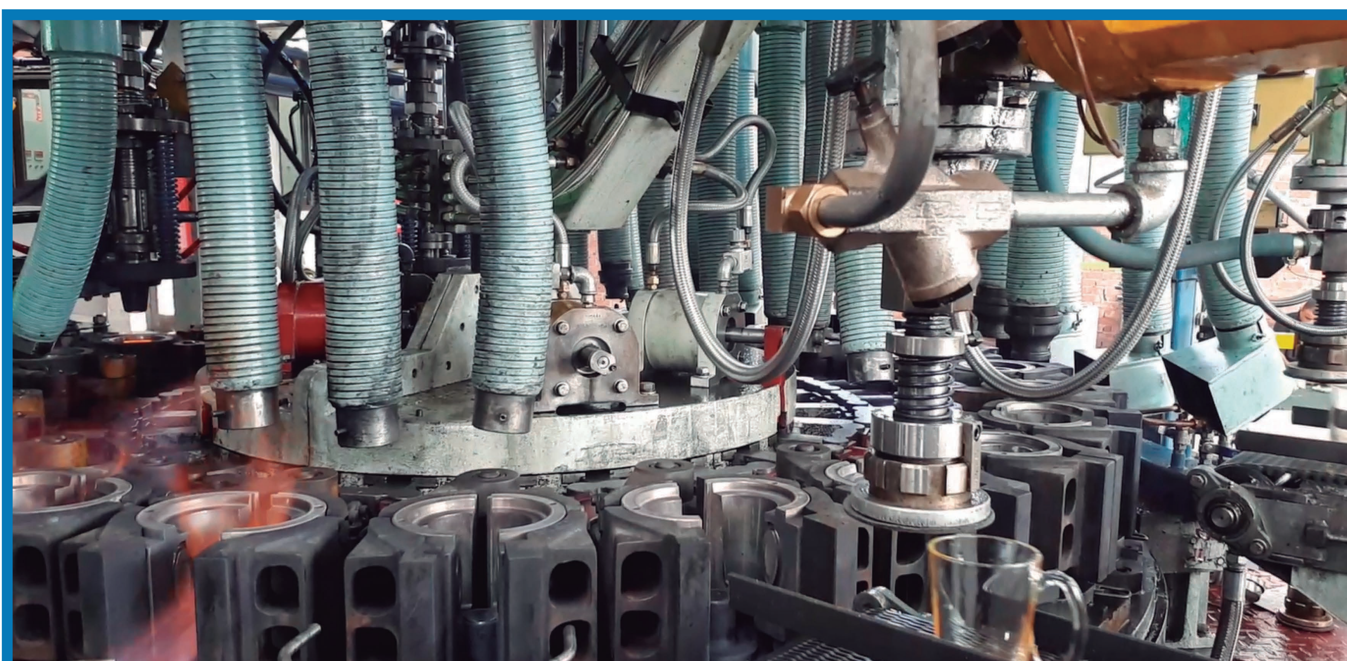
DG SPLIT MOULD SYSTEM IN PRODUCTION - OPENING ANGLE 26°
