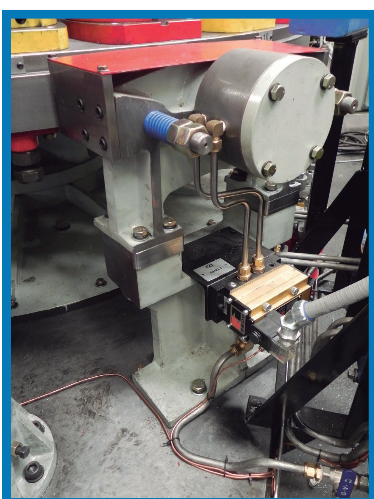
BRAKE MECHANISM
