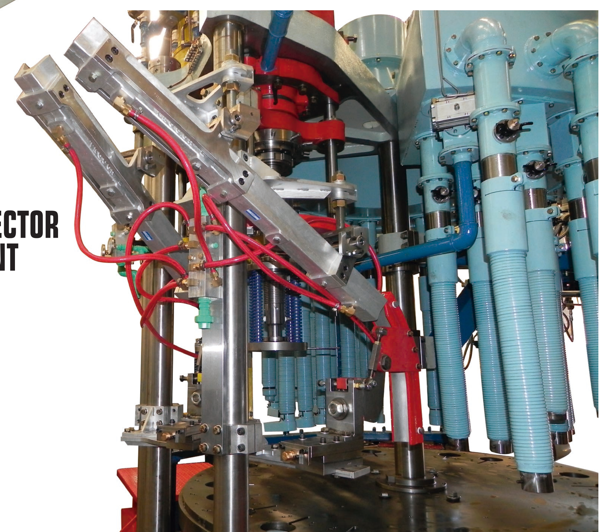
KICK UP MECHANISM
