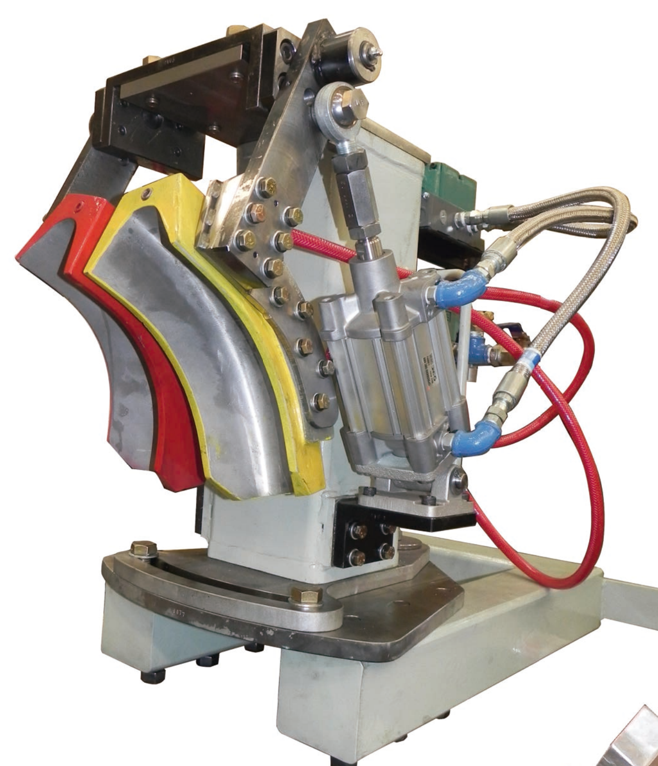
SCOOP MECHANISM
